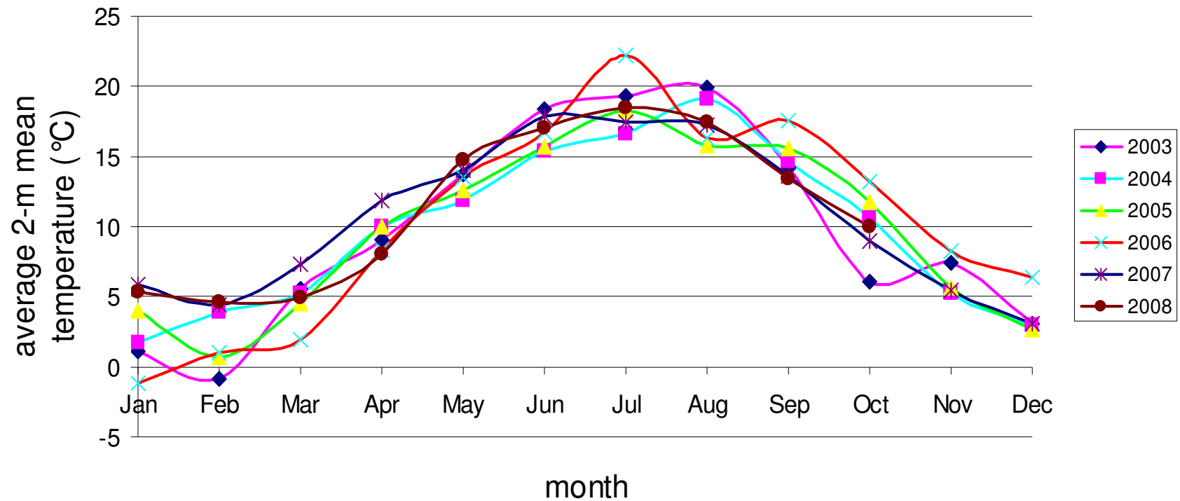
annual 2-m mean temperature
