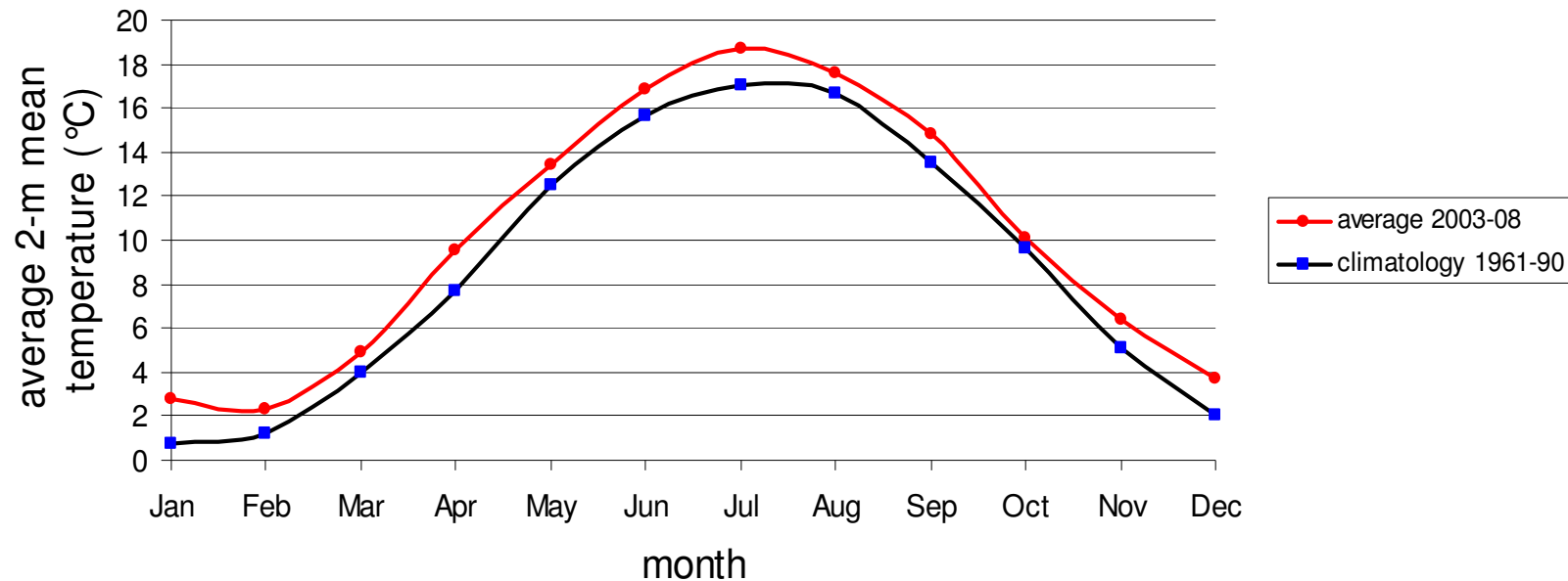
average 2-m mean temperature
