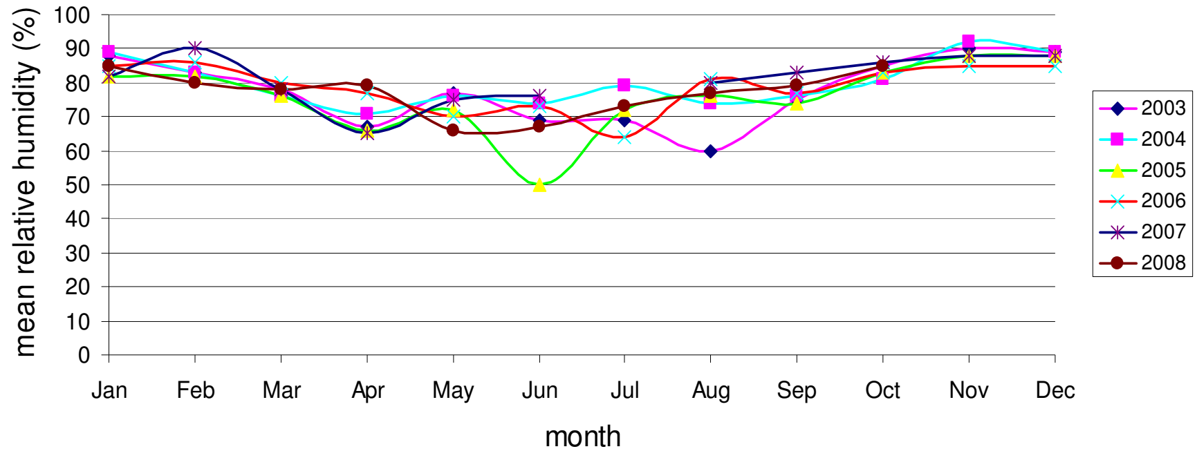
mean relative humidity
