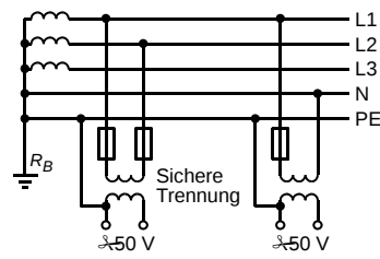
Abb. 25: PELV
